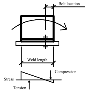
Internal force couple
