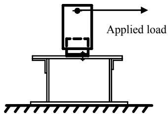
Schematic of Test Setup
