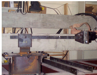
Test Setup
